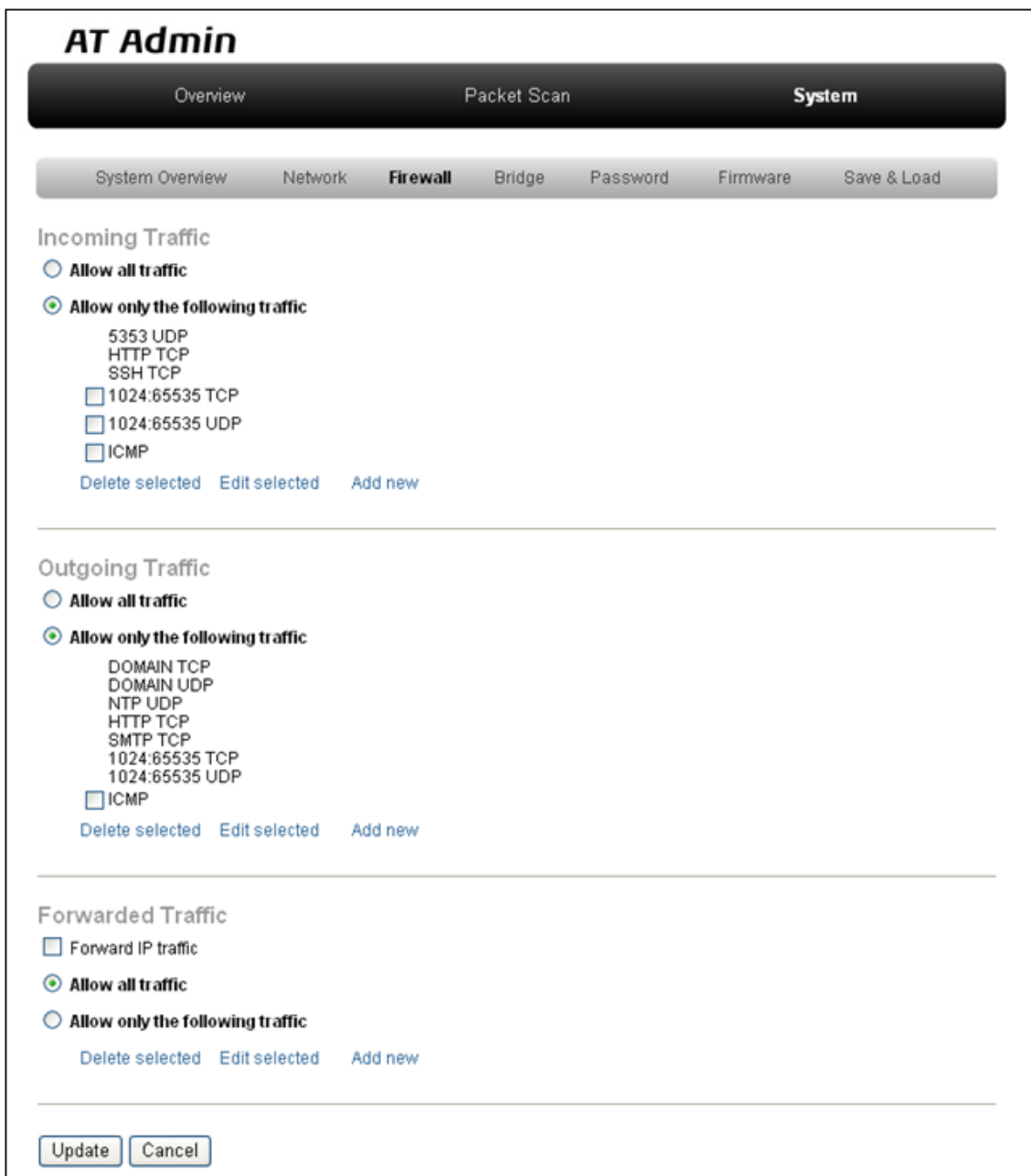
☒ 5.7. AT Admin: System - Firewall
