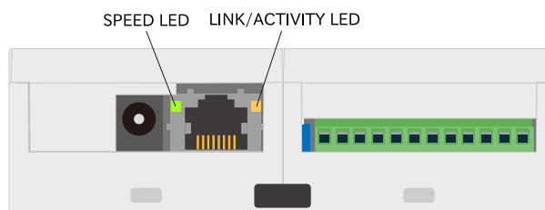
図 3.80 CON2 LAN LED
